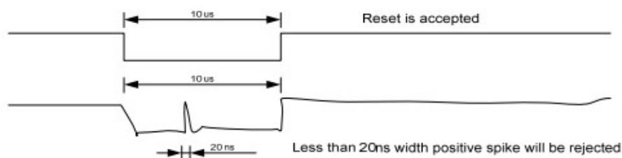
Figure 181: Positive Noise Pulse during Reset Low
